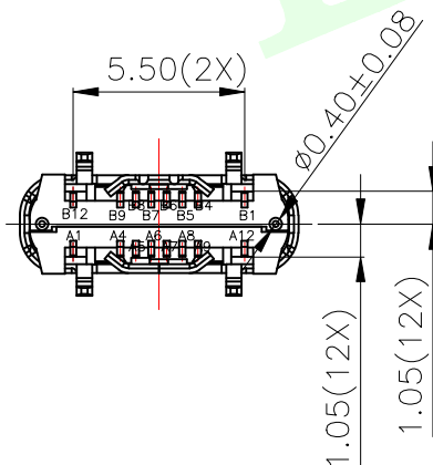
FEMALE AND MALE MATCHING DRAWING
